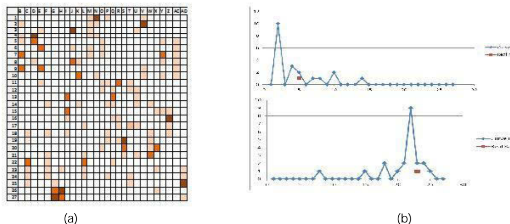
Fig. 4: Ordering distribution for the curves according to the convexity property (a) and a visualisation of the ordering distribution (lines) according to the straightness for two curves shown in Fig. 1 compared to the actual values depicted as fat dots (b).
