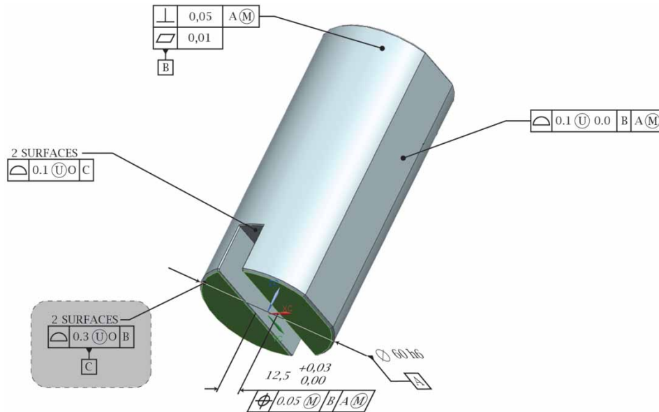
Fig. 3: Model only representation of the case study. Detail of a geometric tolerance query. Tolerance is associated to two features that, together, define the planar datum feature C.
