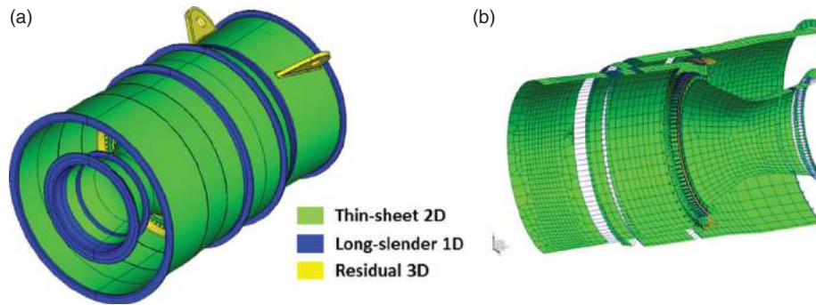
Figure 8. Crescendo engine intermediate casing (a) Cellular decomposition [9], (b) Mixed-dimensional analysis model [10].
