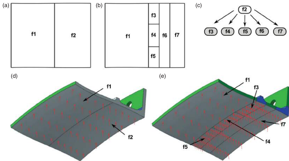
Figure 4. (a) Original solid-fluid interface region; (b) Equivalent interface post model decomposition; (c) Virtual Topology hierarchical relationship between original and decomposed faces; Pressure load on (d) analysis representation of original model; (e) analysis representation of the decomposed model.
