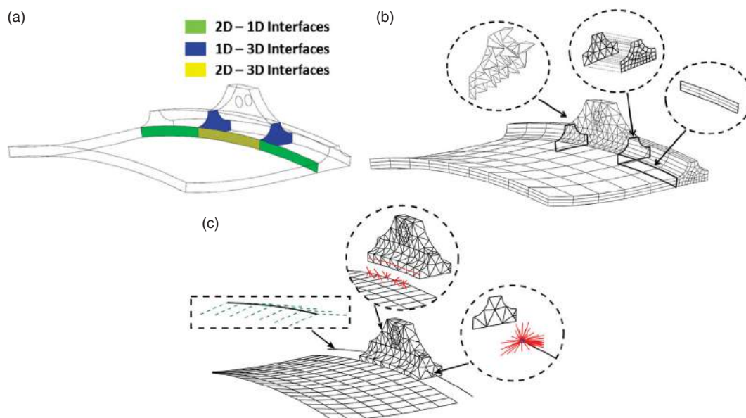
Figure 7. (a) Highlighted interfaces of a section of the aero-casing component; Interface meshing for (b) mixed-solid mesh; (c) mixed-dimensional mesh.
