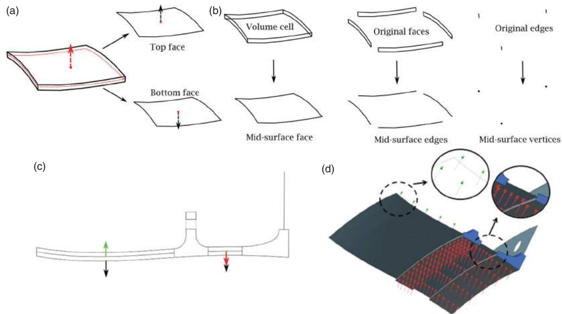
Figure 6. (a) Thin-sheet region and defining face pairs of mid-surface; (b) Equivalence dependencies for mid-surface representation; (c) Comparison of surface normals between face pairs and their equivalent mid-surface face (d) Pressure load on mixed-dimensional model with correct orientations.
