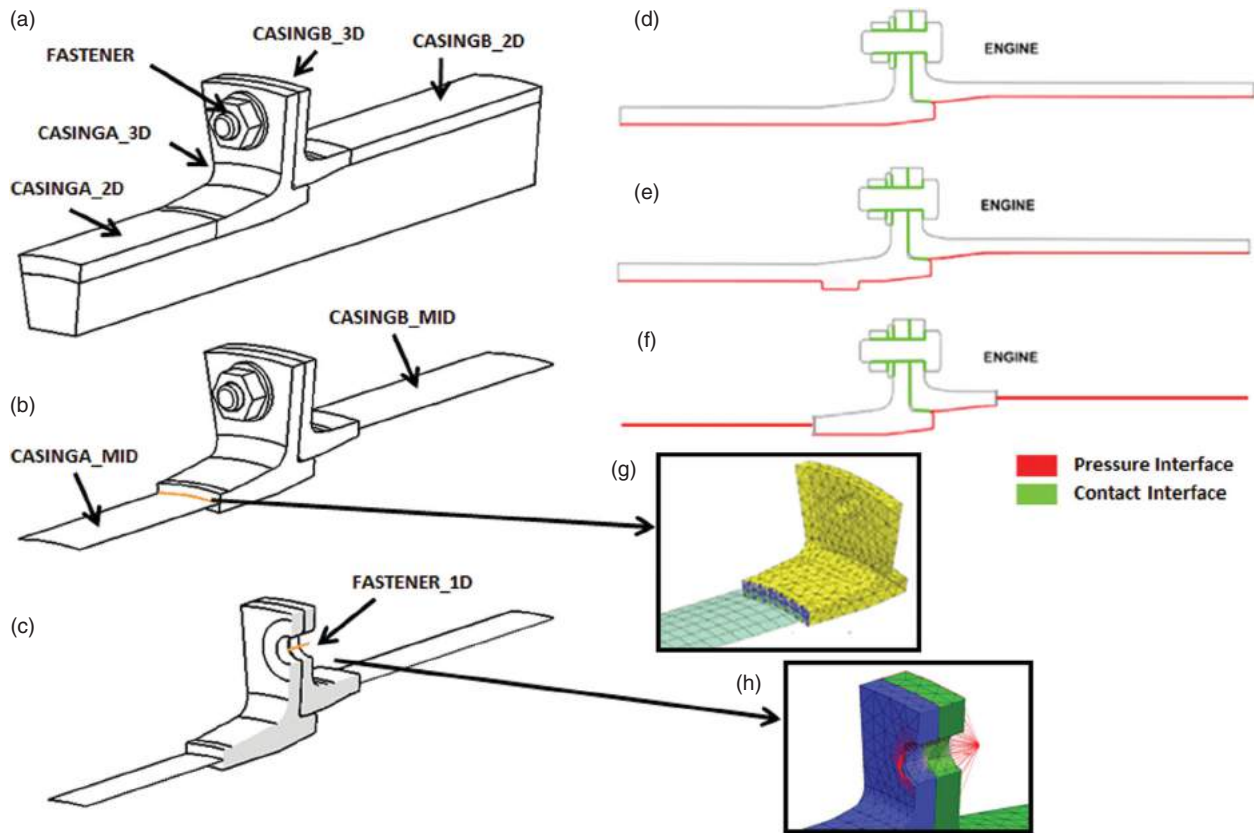
Figure 9. (a) Decomposed cyclic symmetric sector of bolted flange; (b) 2D idealization of thin-sheet ('_2D') regions; (c) 1D idealization of fastener assembly; Interfaces in: (d) 3D representation; (e) 3D representation after design changes; (f) 2D idealization; (g) 2D-3D coupling; (h) 1D-3D coupling.
