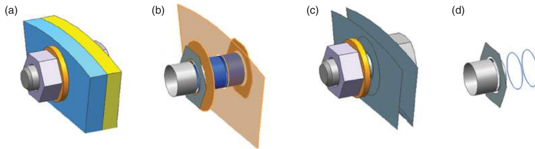
Figure 1. (a) 3D fastened plate assembly; (b) Interfaces in 3D fastened plate assembly; (c) Mid-surface representation of fastened plate assembly; (d) Interfaces in dimensionally-reduced fastened plate assembly.
