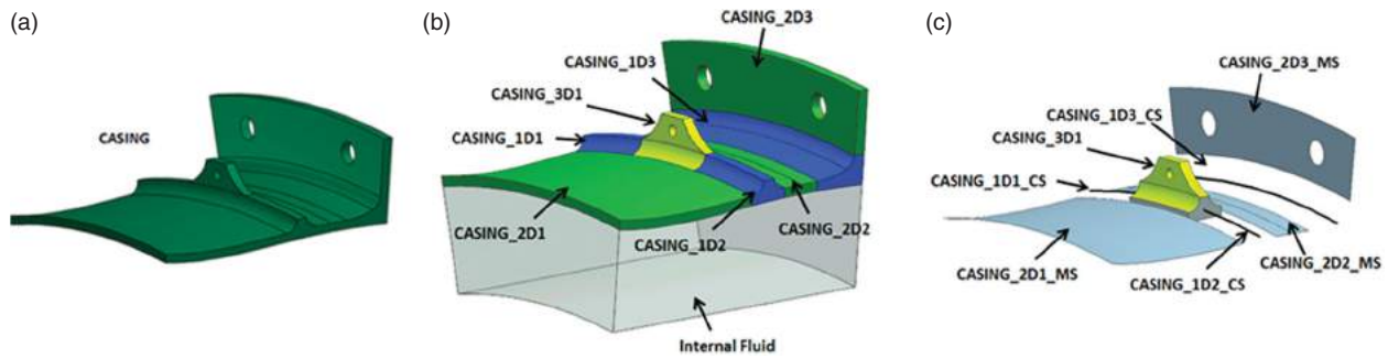
Figure 3. (a) Aero-casing section; (b) Cellular model of 3D analysis decomposition; (c) Lower fidelity mixed-dimensional model.
