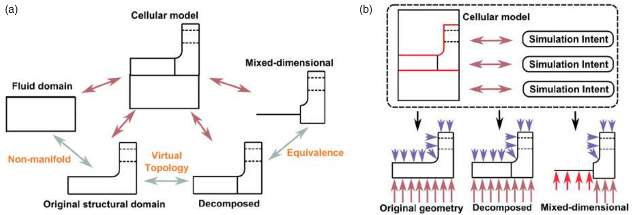
Figure 2. (a) Technologies used to link analysis representations; (b) Linking with Simulation Intent to create fit-for-purpose analysis models at different levels of fidelity.
