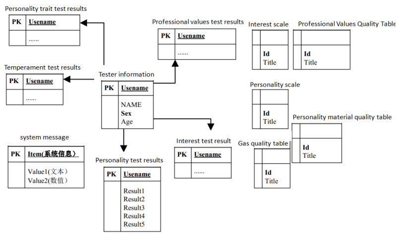
Figure 7: Relationship between data tables.
