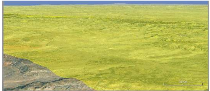
Fig. 7(b): After zooming in on a portion of an edge.
