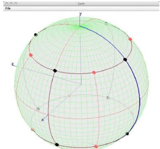
Fig. 5(b): First level of subdivision.
