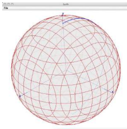
Fig. 2: Three orthogonal families of plane slices. The blue line leaving the North Pole is the International Date Line.
