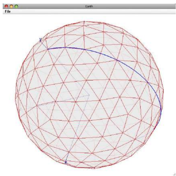
Fig. 3(b): After two refinement steps.
