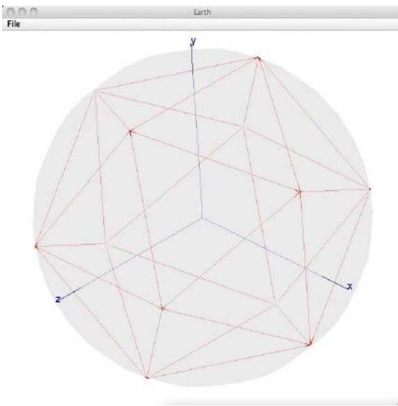
Fig. 3(a): An icosahedron inscribed in the ellipsoid.
