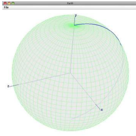
Fig. 4: A tessellation based on generating quadrilaterals aligned with latitude and longitude lines.
