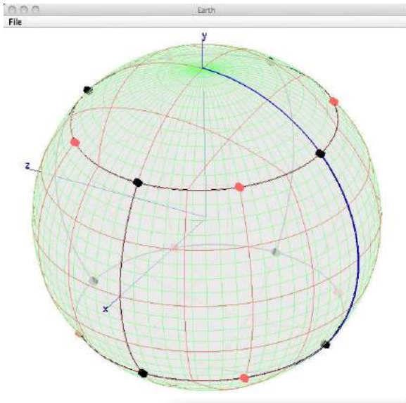
Fig. 5(c): Second level of subdivision
