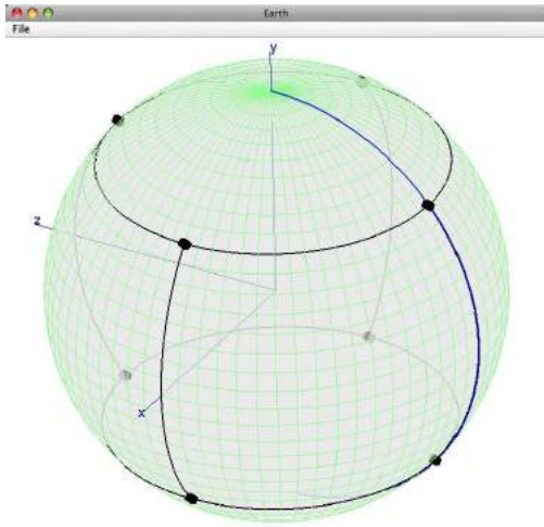
Fig. 5(a): Mapping a cube onto the globe.
