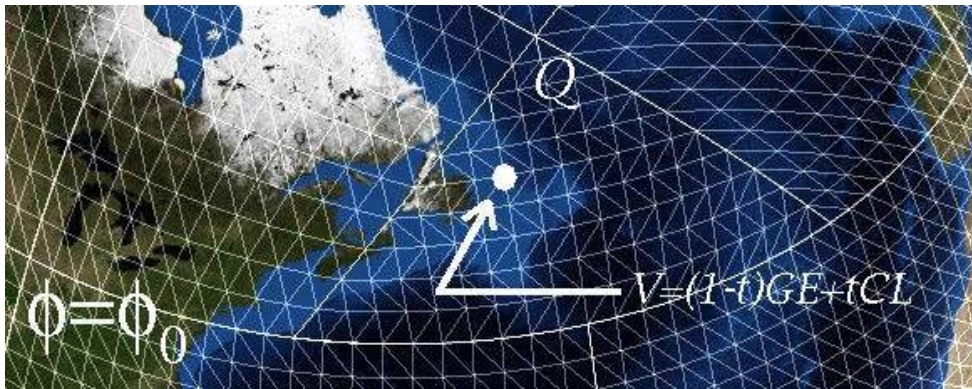
Fig. 6: An area where the polar region meets the lateral sides of the globe.
