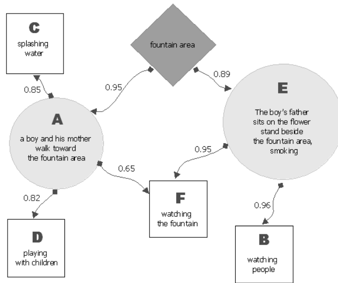
Fig. 5: The expression method of the activity model in the commonsense knowledge model. The circle represents the sensor node. The behavior detected by a set of sensors is corresponded to a sensor node. The rectangle represents the behavior node, the behavior inferred by the sensor node and the location node. The rhombus represents the location node. The location detected by a set of sensors is corresponded to a location node. The connective arrowhead represents the relationships between the nodes. The direction to which the arrowhead point is the child node, and the other end of the arrow is the father node.
